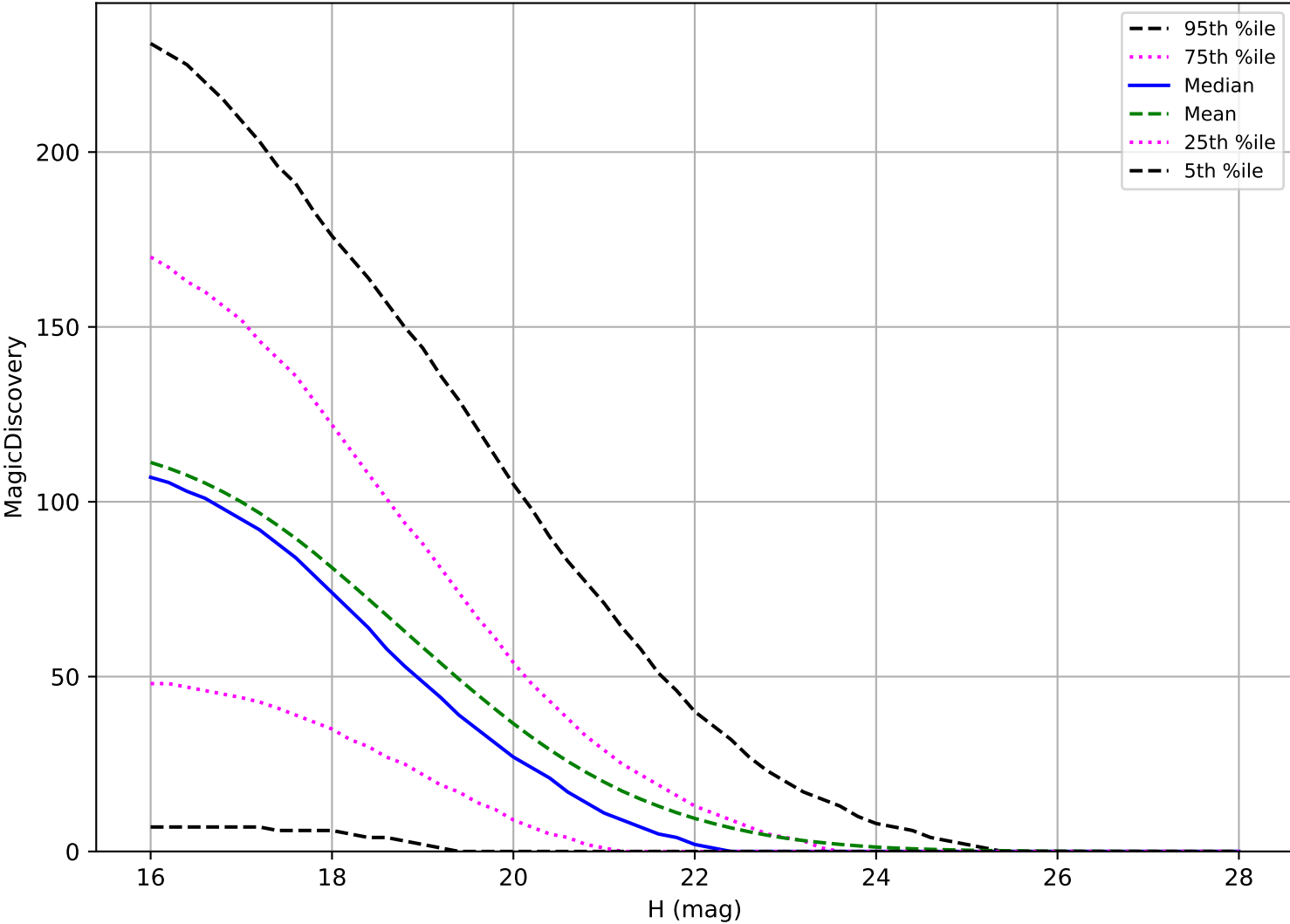
ddf_acor_sf10_lsf15_lsr20_v3.4_10yrs: PHA 6 detections in 60 nights detection loss
