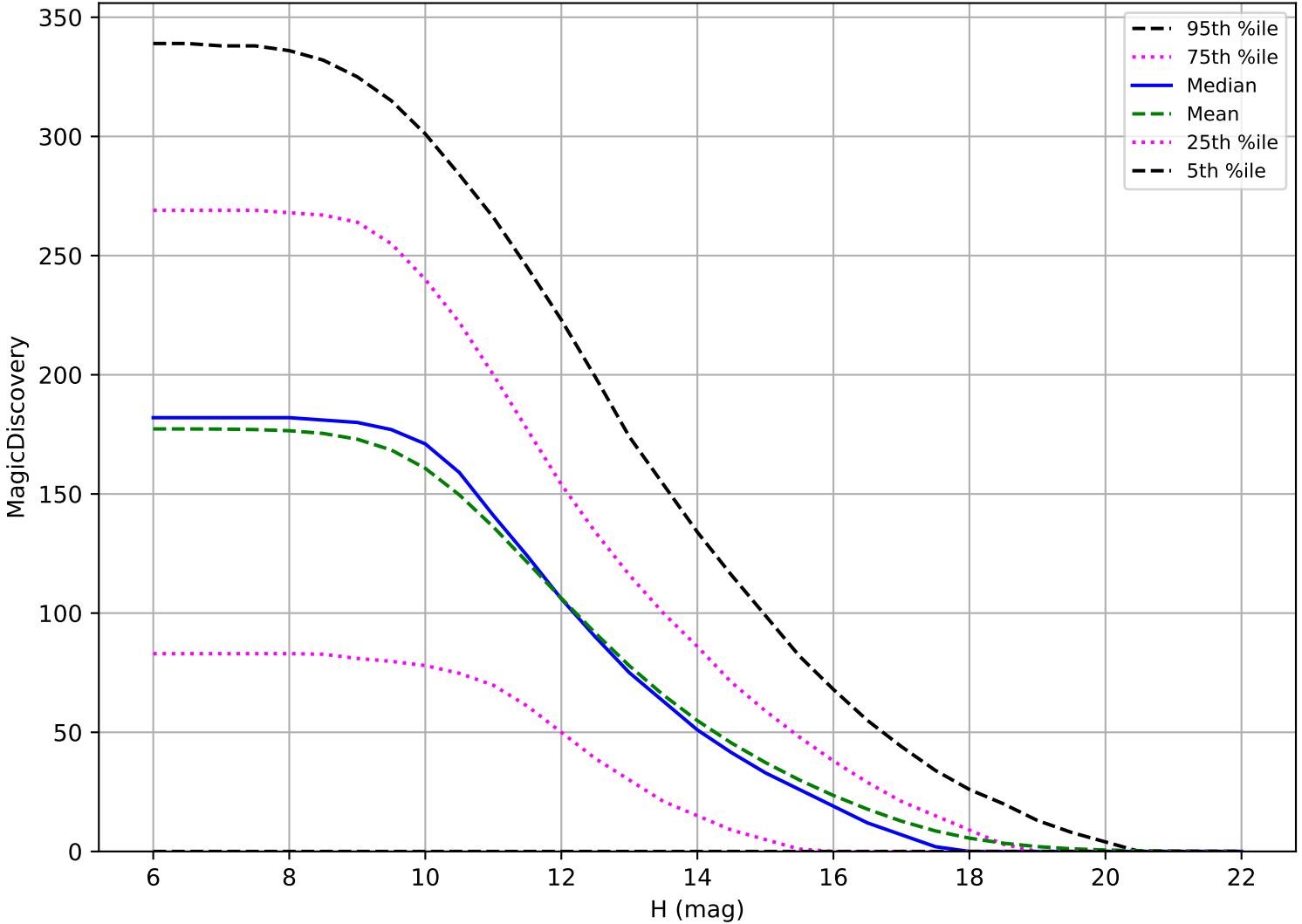
ddf_acor_sf10_lsf15_lsr20_v3.4_10yrs: OCC_r5 6 detections in 60 nights detection loss
