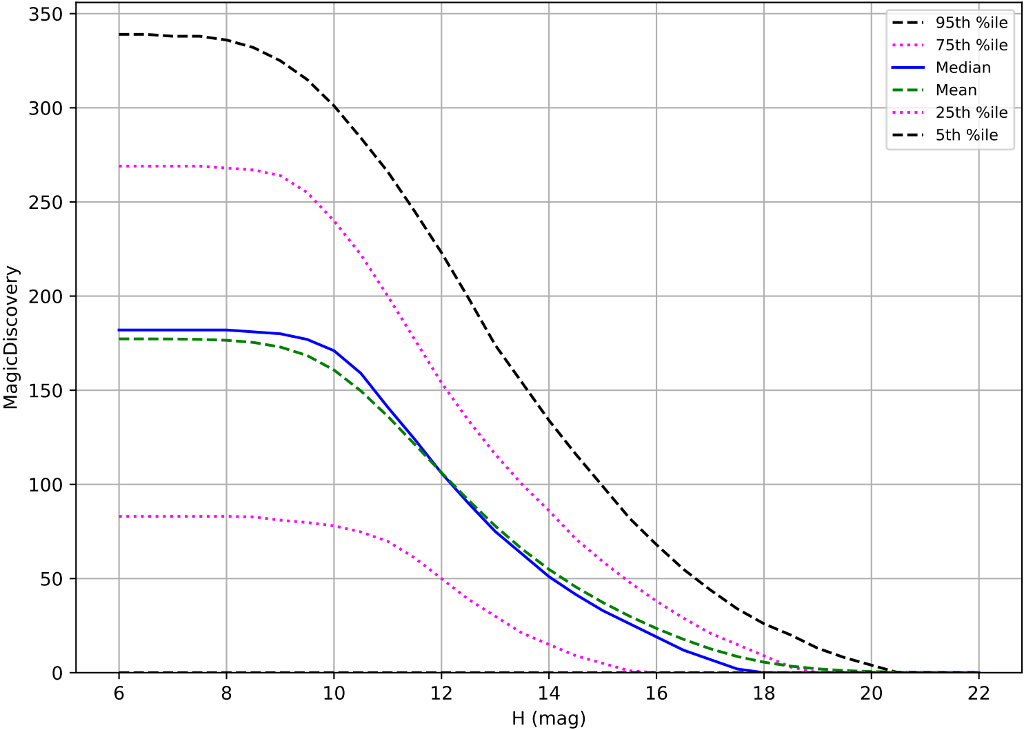
ddf_acor_sf10_lsf15_lsr20_v3.4_10yrs: OCC_r5 6 detections in 60 nights detection loss
