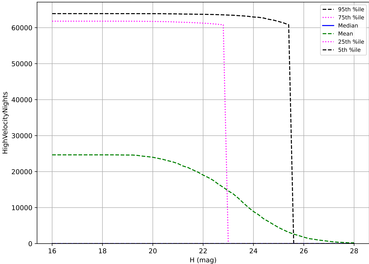
ddf_acor_sf10_lsf15_lsr20_v3.4_10yrs: PHA High velocity pair detection loss
