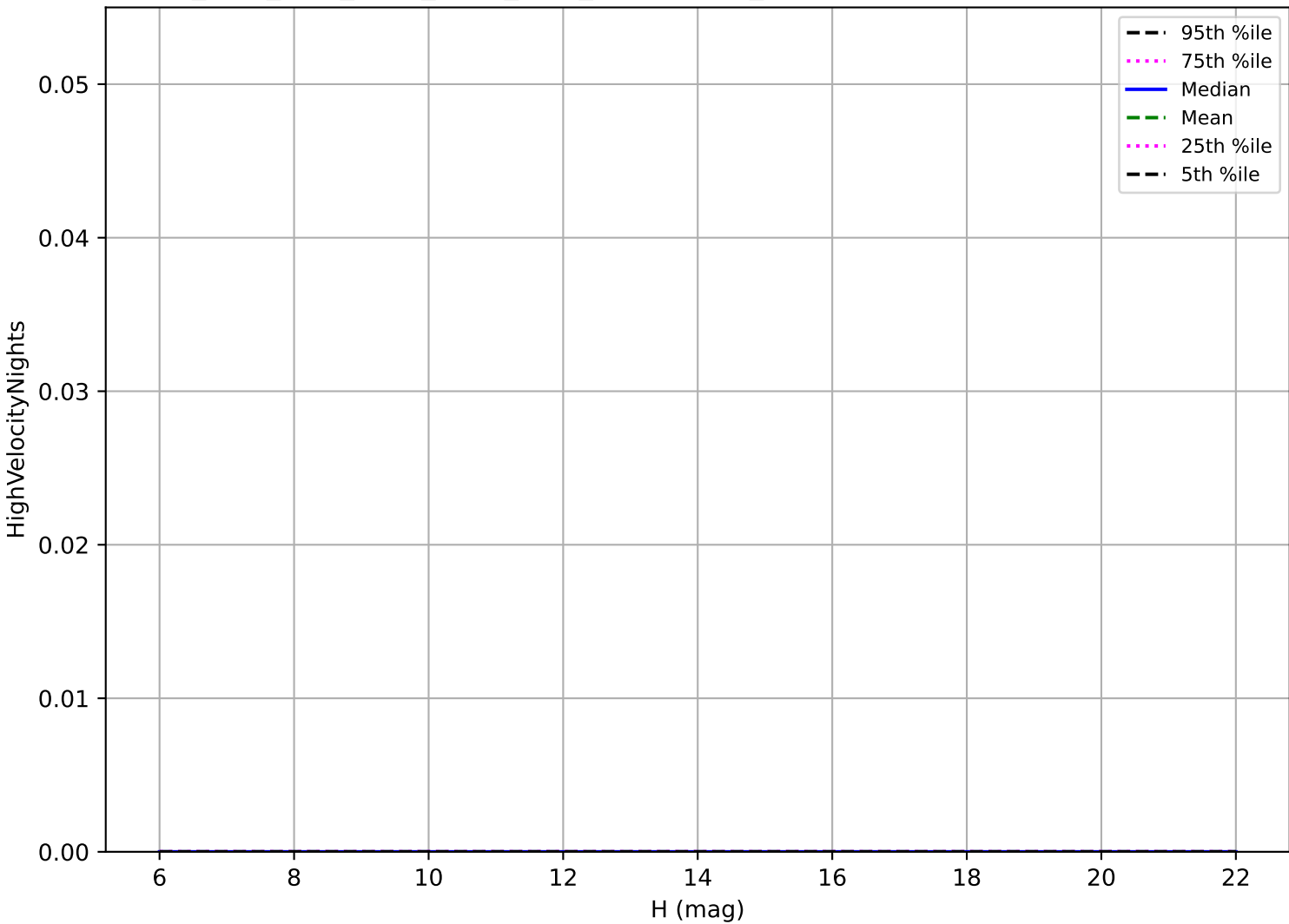
ddf_acor_sf10_lsf15_lsr20_v3.4_10yrs: OCC_r5 High velocity pair detection loss
