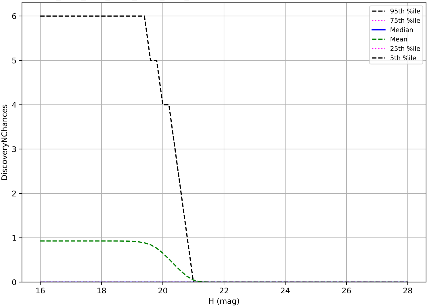
ddf_acor_sf10_lsf15_lsr20_v3.4_10yrs: Vatira 3 pairs in 15 nights detection loss
