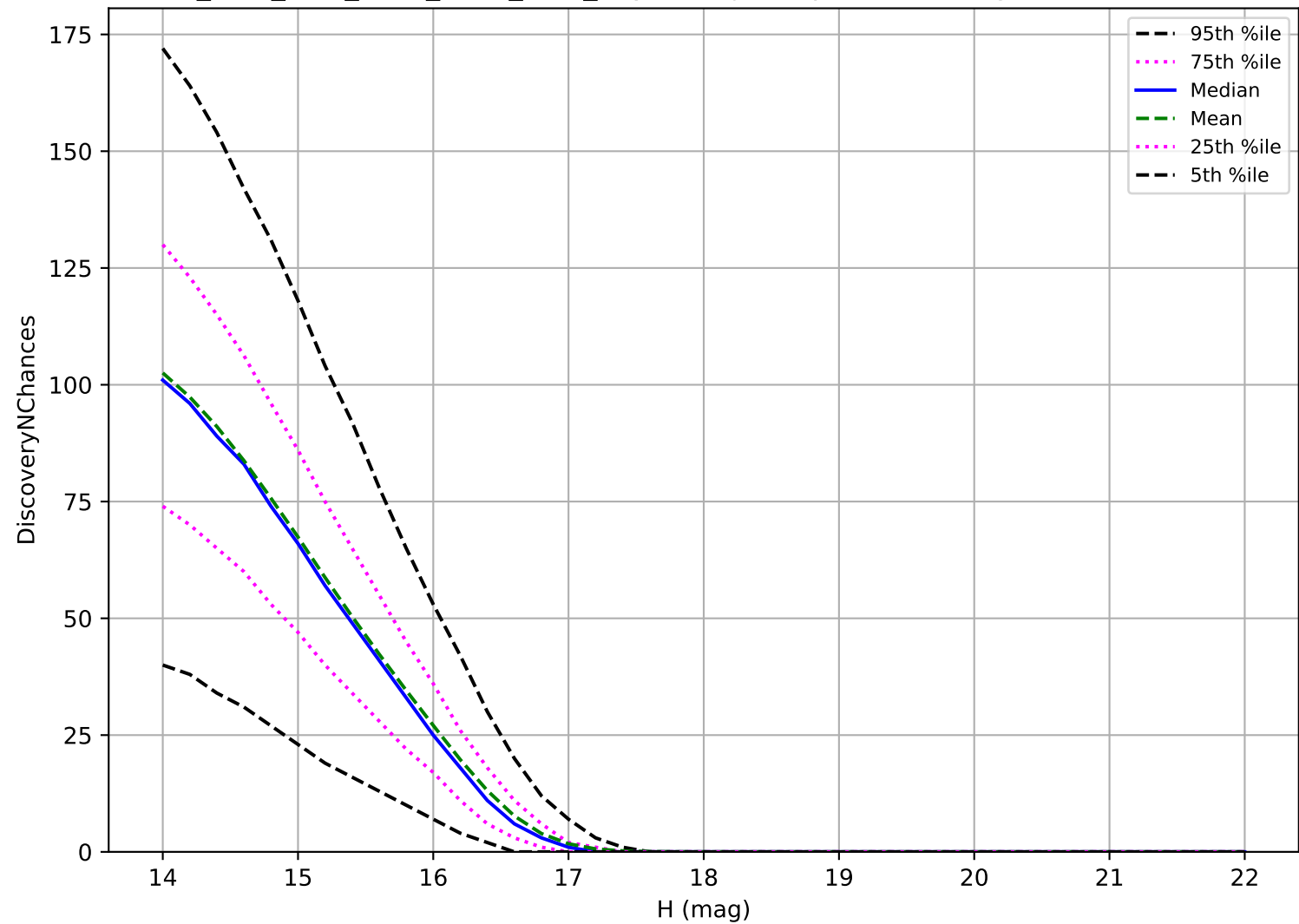
ddf_acor_sf10_lsf15_lsr20_v3.4_10yrs: Trojan 3 pairs in 15 nights detection loss
