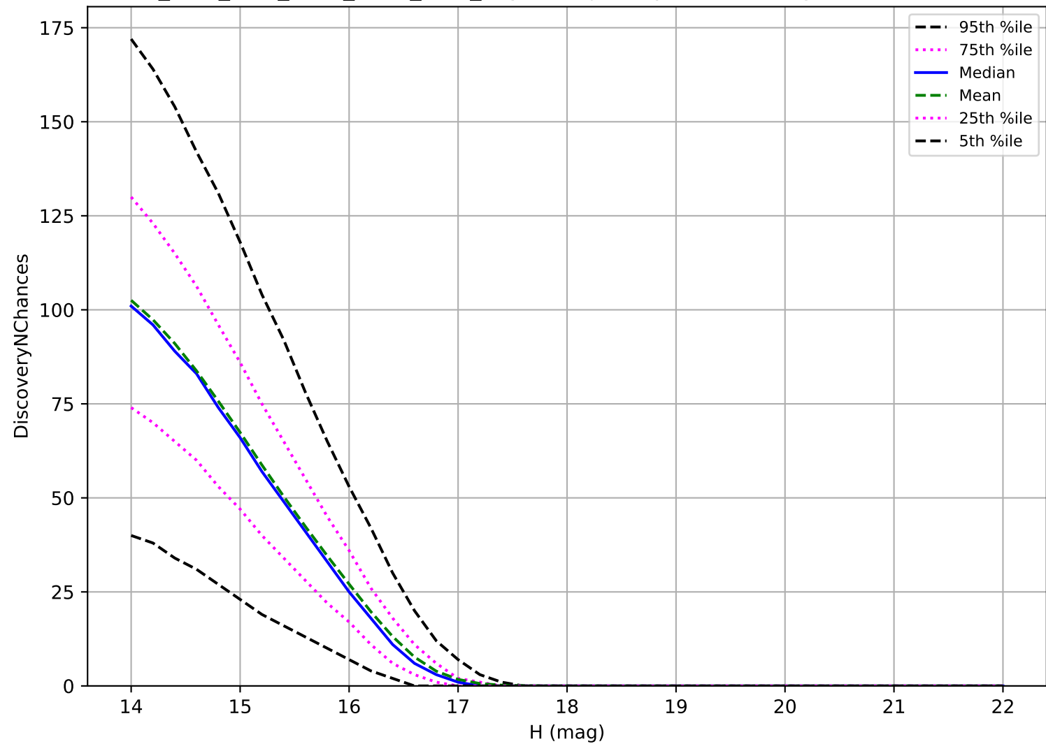
ddf_acor_sf10_lsf15_lsr20_v3.4_10yrs: Trojan 3 pairs in 15 nights detection loss
