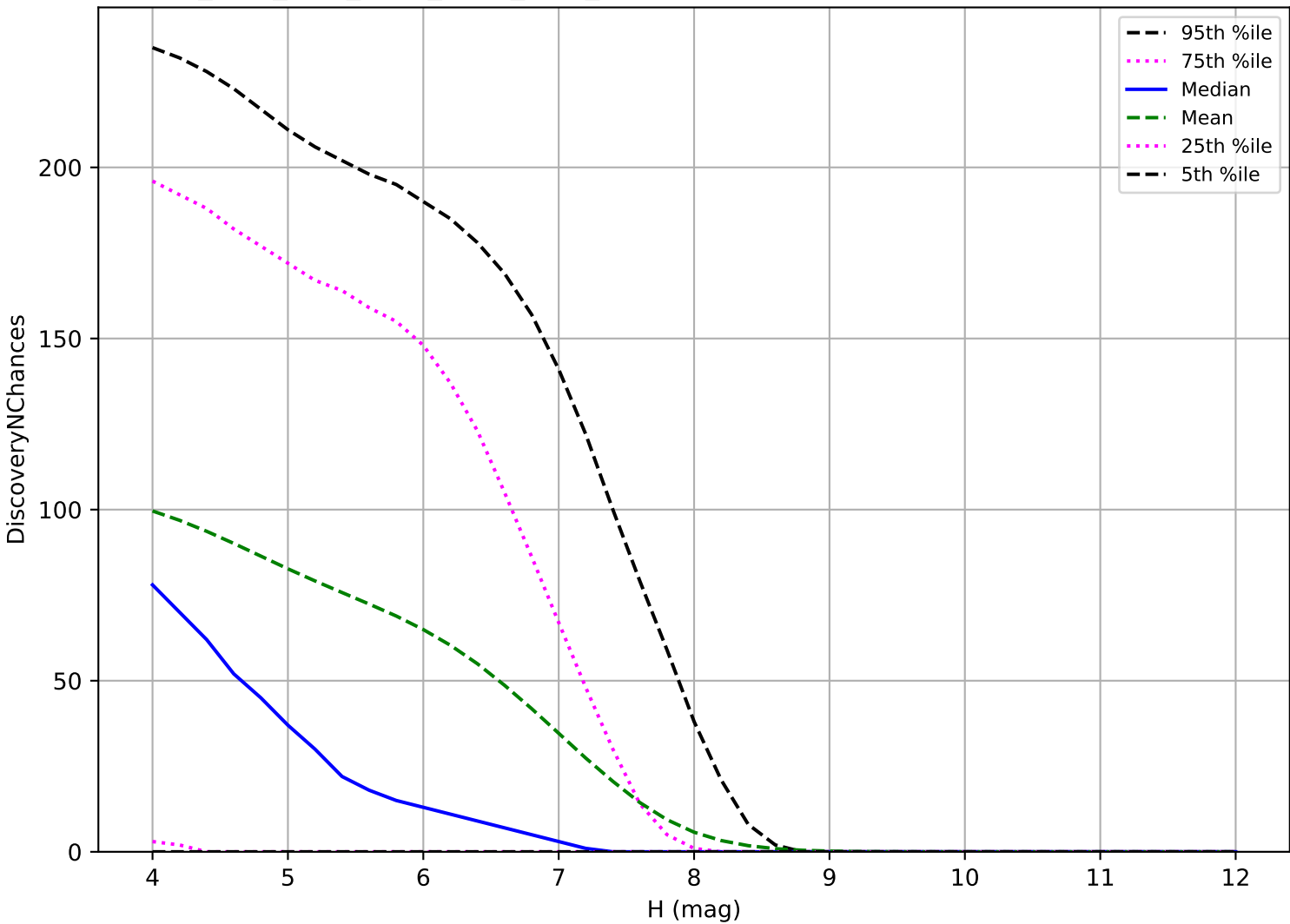
ddf_acor_sf10_lsf15_lsr20_v3.4_10yrs: TNO 3 pairs in 15 nights detection loss
