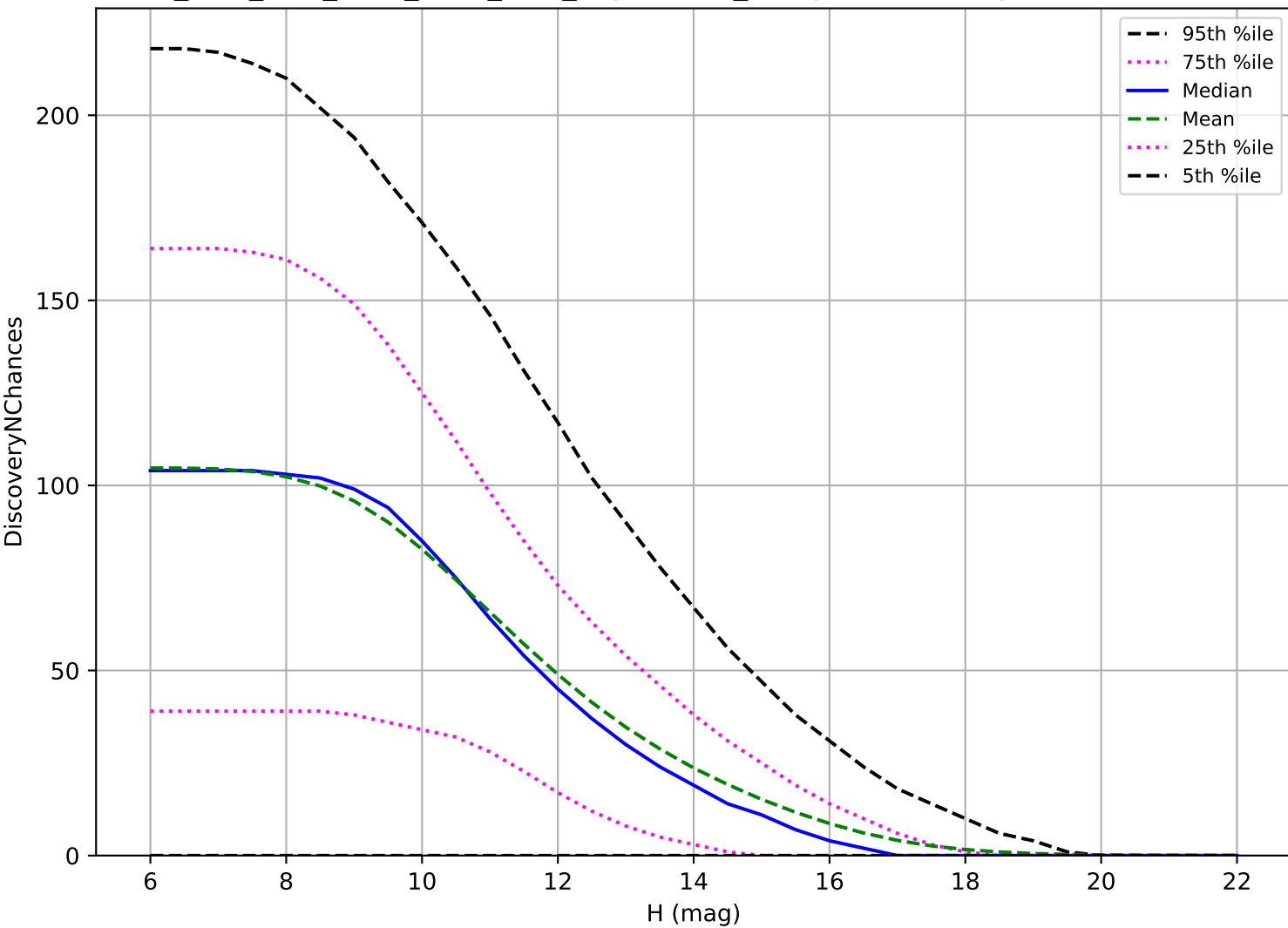
ddf_acor_sf10_lsf15_lsr20_v3.4_10yrs: OCC_r5 3 pairs in 15 nights detection loss
