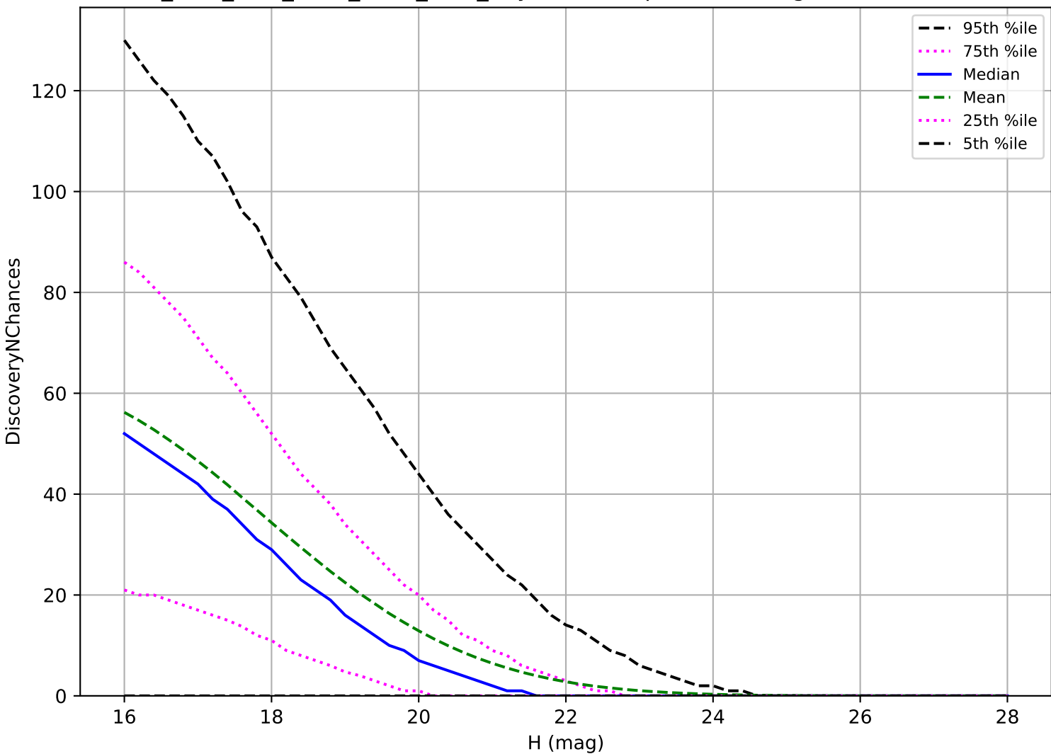
ddf_acor_sf10_lsf15_lsr20_v3.4_10yrs: NEO 3 pairs in 15 nights detection loss
