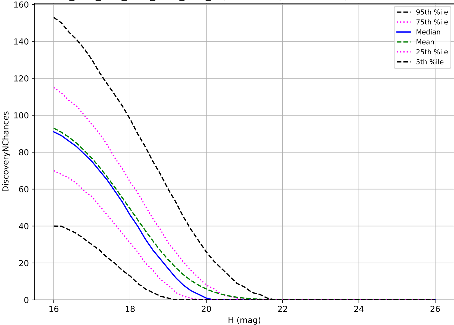
ddf_acor_sf10_lsf15_lsr20_v3.4_10yrs: MBA 3 pairs in 15 nights detection loss
