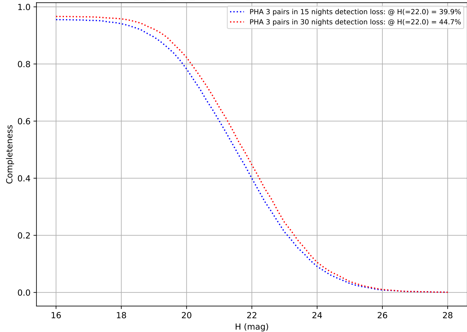
ddf_acor_sf10_lsf15_lsr20_v3.4_10yrs: DifferentialCompleteness
