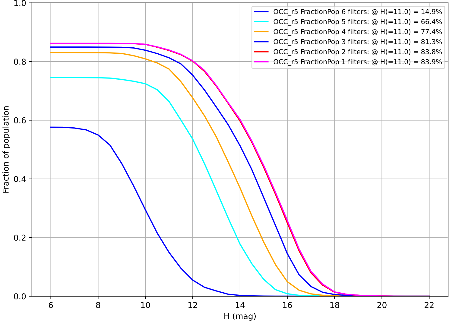
ddf_acor_sf10_lsf15_lsr20_v3.4_10yrs: Fraction of population with colors in X filters OCC_r5
