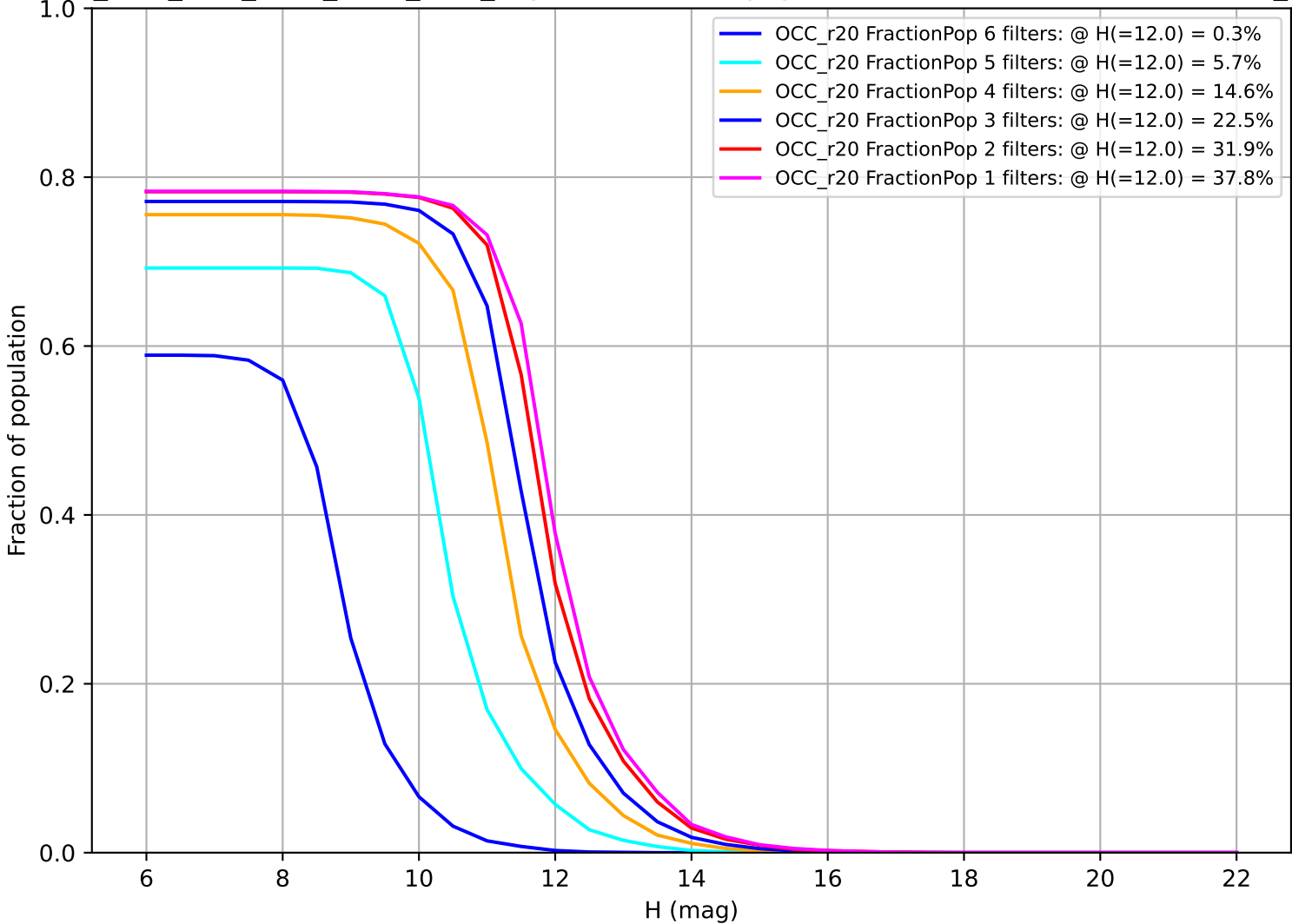
ddf_acor_sf10_lsf15_lsr20_v3.4_10yrs: Fraction of population with colors in X filters OCC_r20
