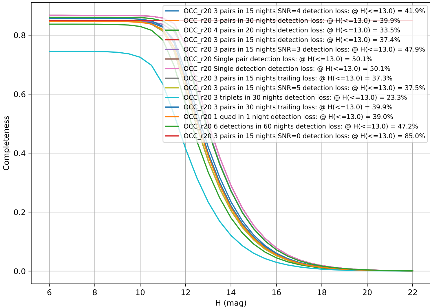
ddf_acor_sf10_lsf15_lsr20_v3.4_10yrs: CumulativeCompleteness
