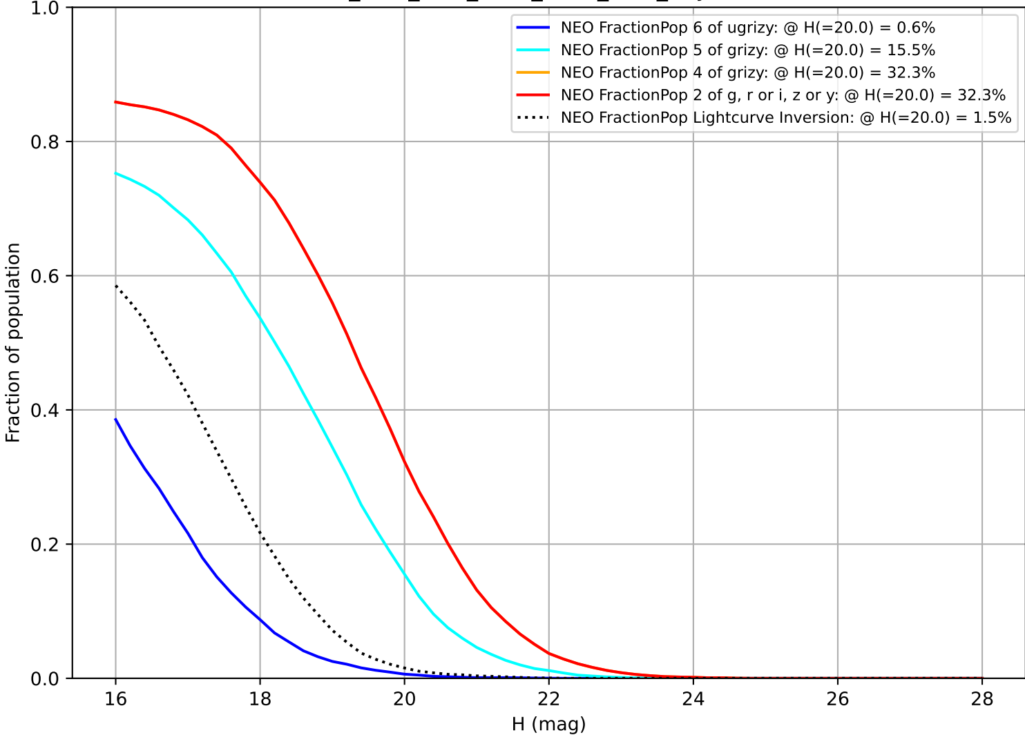
ddf_acor_sf10_lsf15_lsr20_v3.4_10yrs NEO
