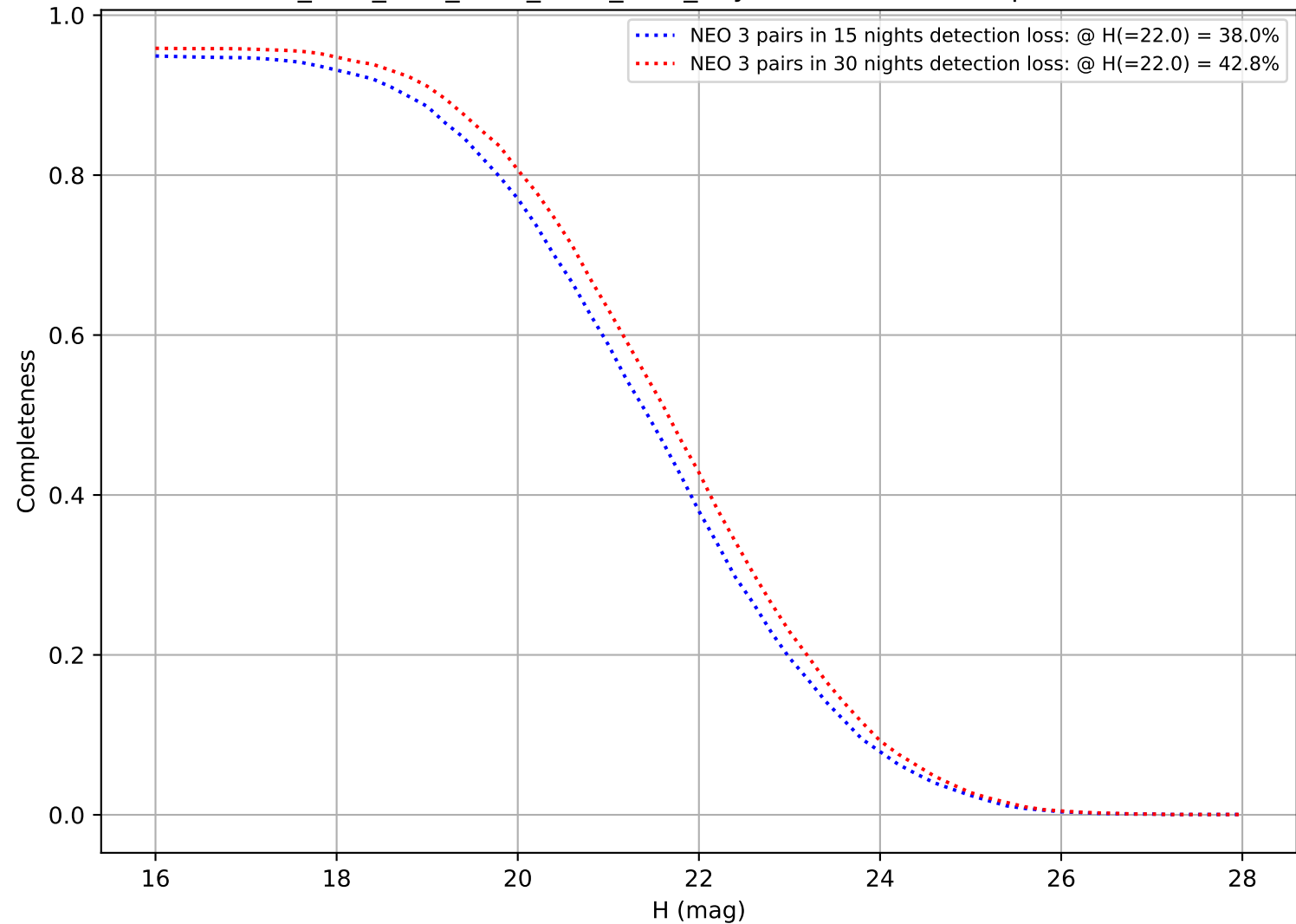
ddf_acor_sf10_lsf15_lsr20_v3.4_10yrs: DifferentialCompleteness
