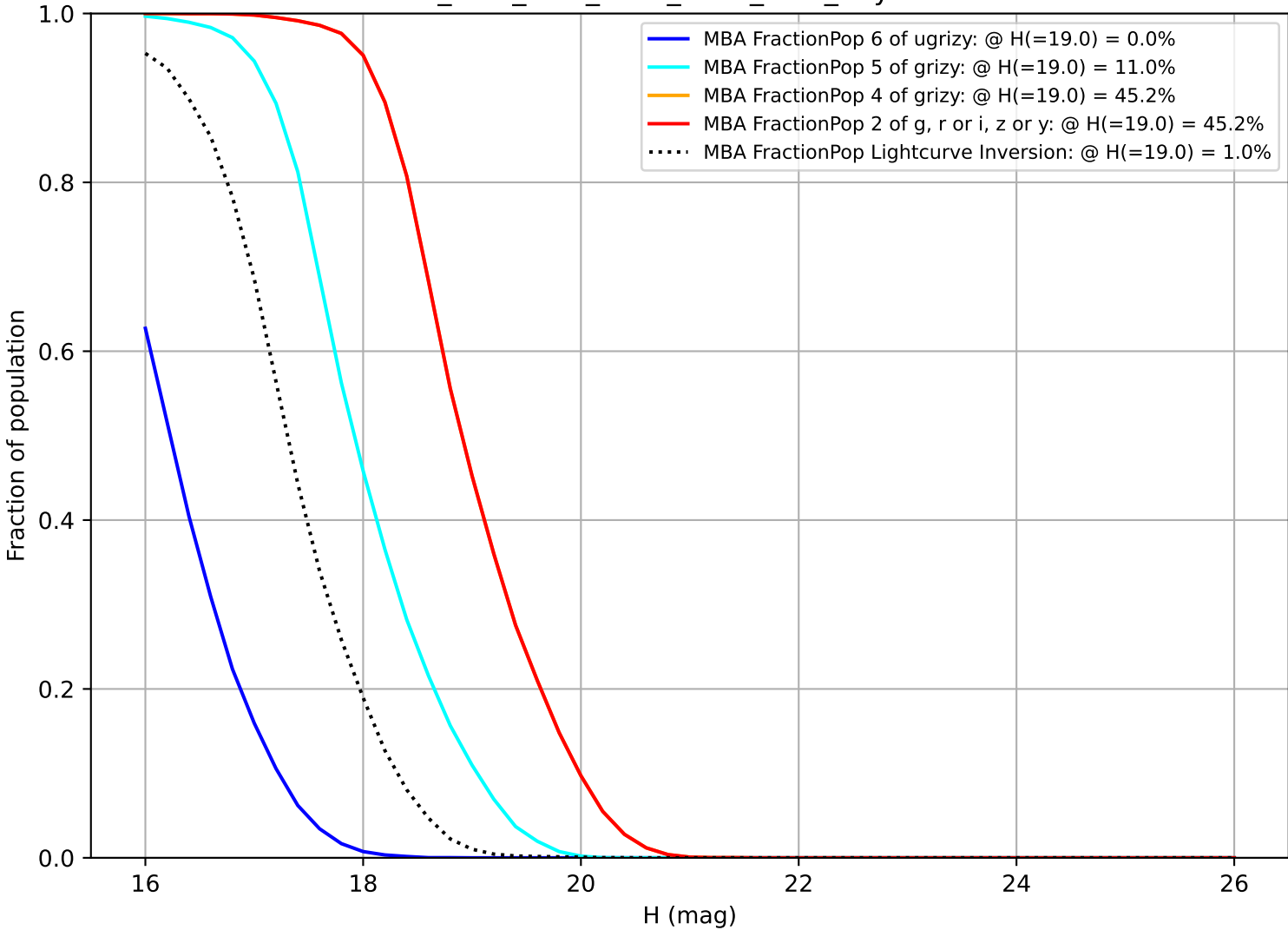
ddf_acor_sf10_lsf15_lsr20_v3.4_10yrs MBA
