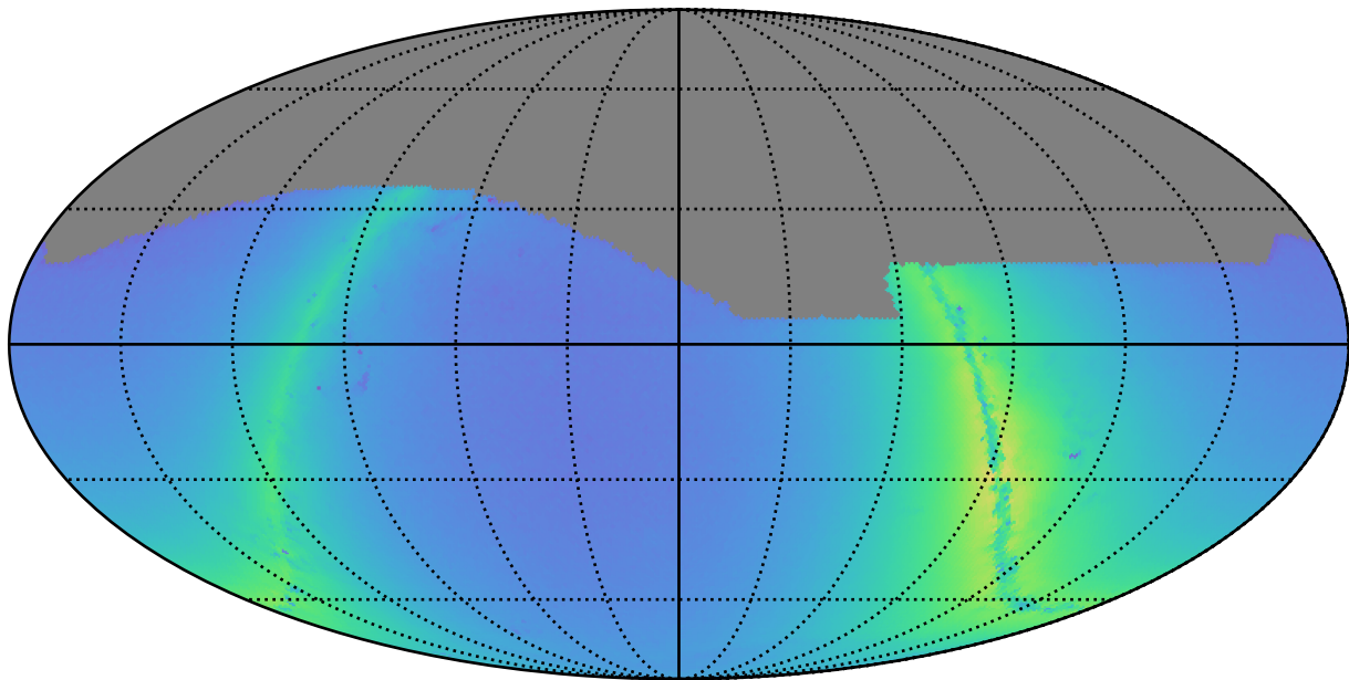
ddf_acor_sf10_lsf15_lsr20_v3.4_10yrs r: Nstars_no_crowding
