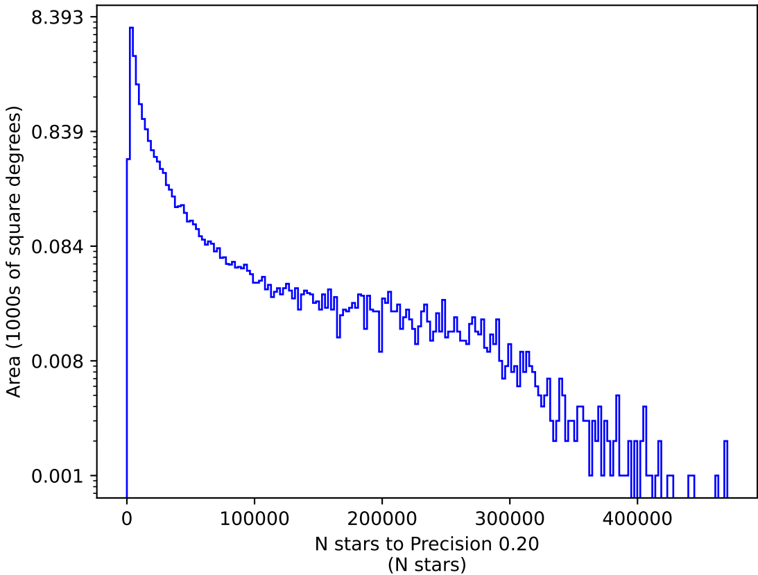
ddf_acor_sf10_ls15_lsr20_v3.4_10yrs u: N stars to Precision 0.20
