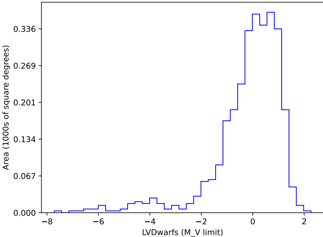
ddf_acor_sf10_lsf15_lsr20_v3.4_10yrs gi SCP: LVDwarfs
