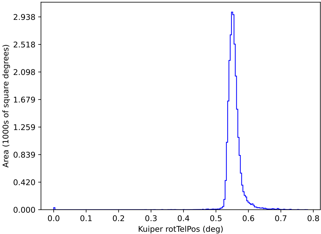
ddf_acor_sf10_lsf15_lsr20_v3.4_10yrs y: Kuiper rotTelPos
