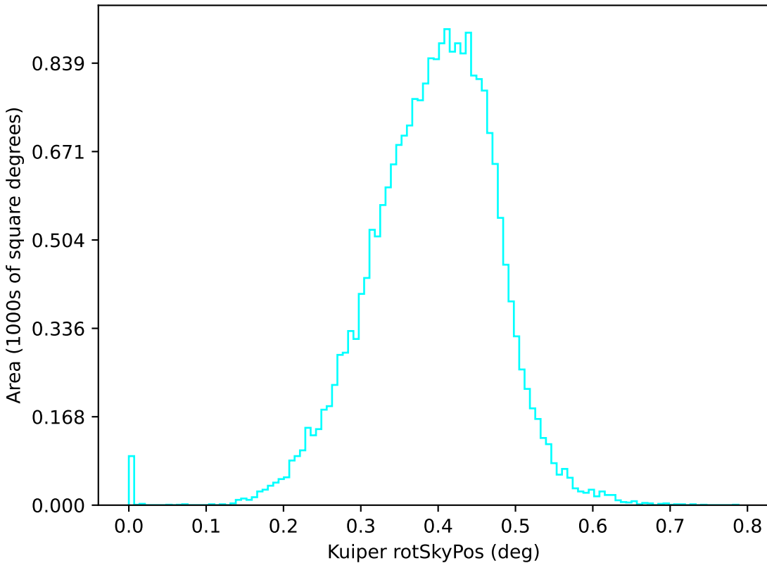
ddf_acor_sf10_lsf15_lsr20_v3.4_10yrs u: Kuiper rotSkyPos
