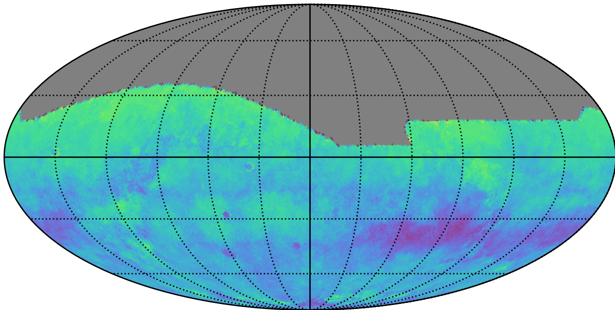
ddf_acor_sf10_lsf15_lsr20_v3.4_10yrs r: Kuiper rotSkyPos
