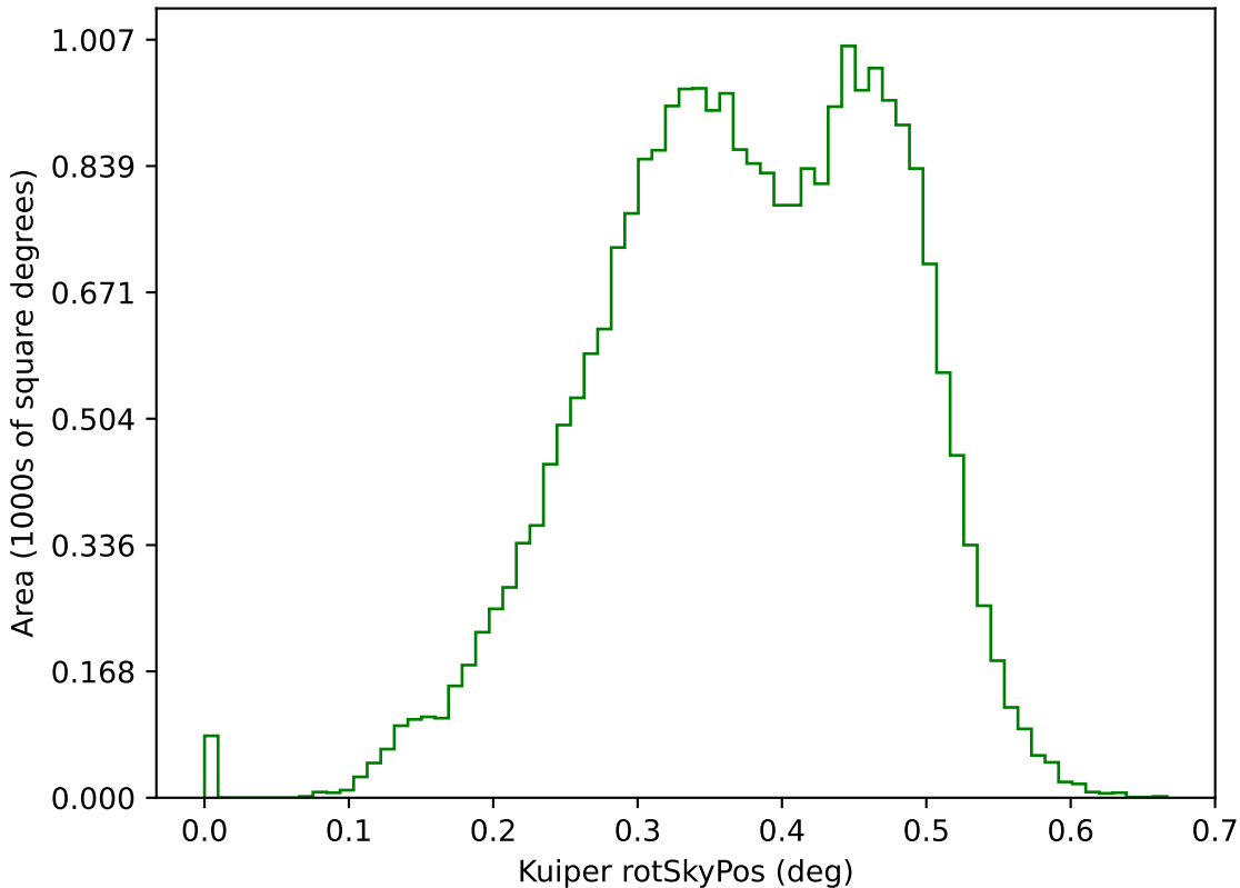
ddf_acor_sf10_lsf15_lsr20_v3.4_10yrs g: Kuiper rotSkyPos
