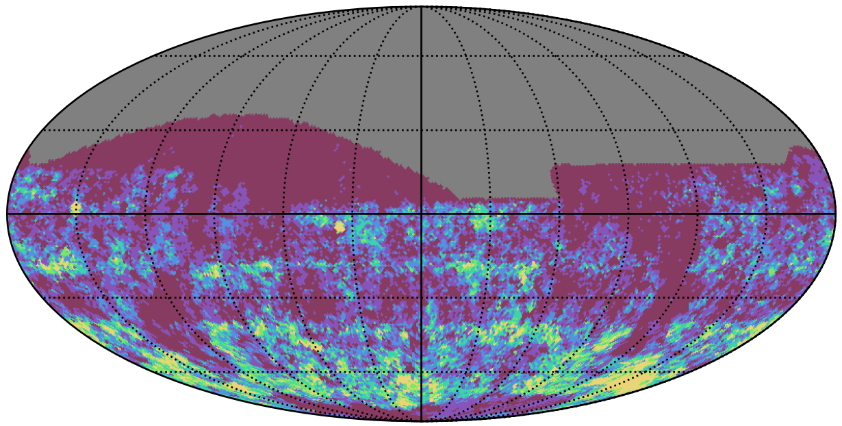
ddf_acor_sf10_lsf15_lsr20_v3.4_10yrs r band: Gaps_3hr
