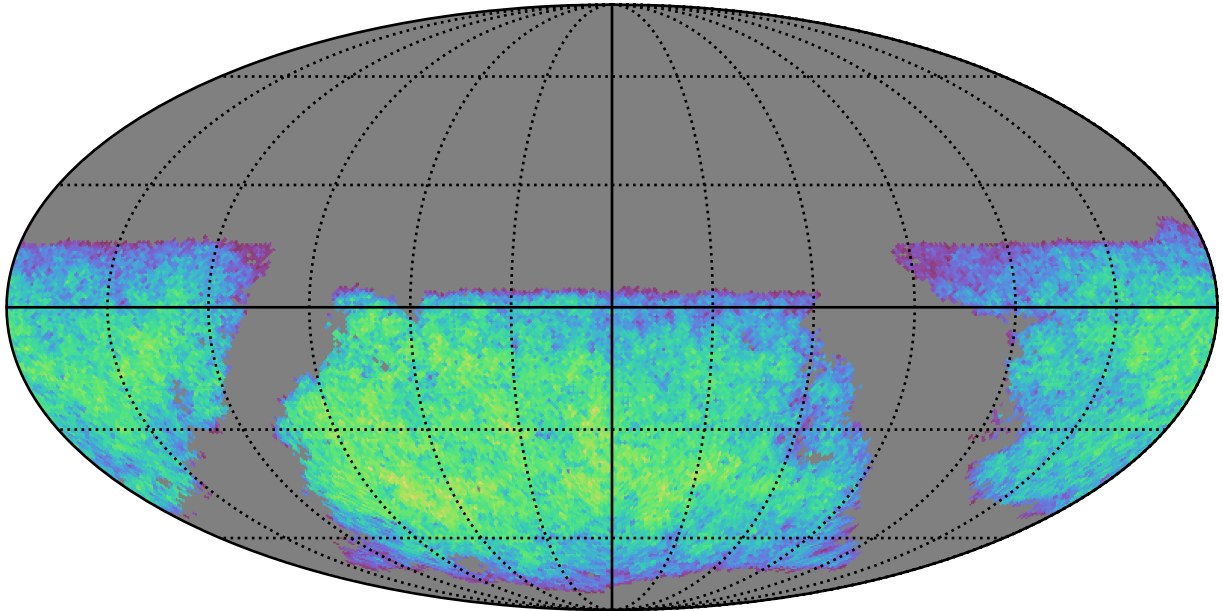
ddf_acor_sf10_lsf15_lsr20_v3.4_10yrs i band non-DD year 1: ExgalM5WithCuts
