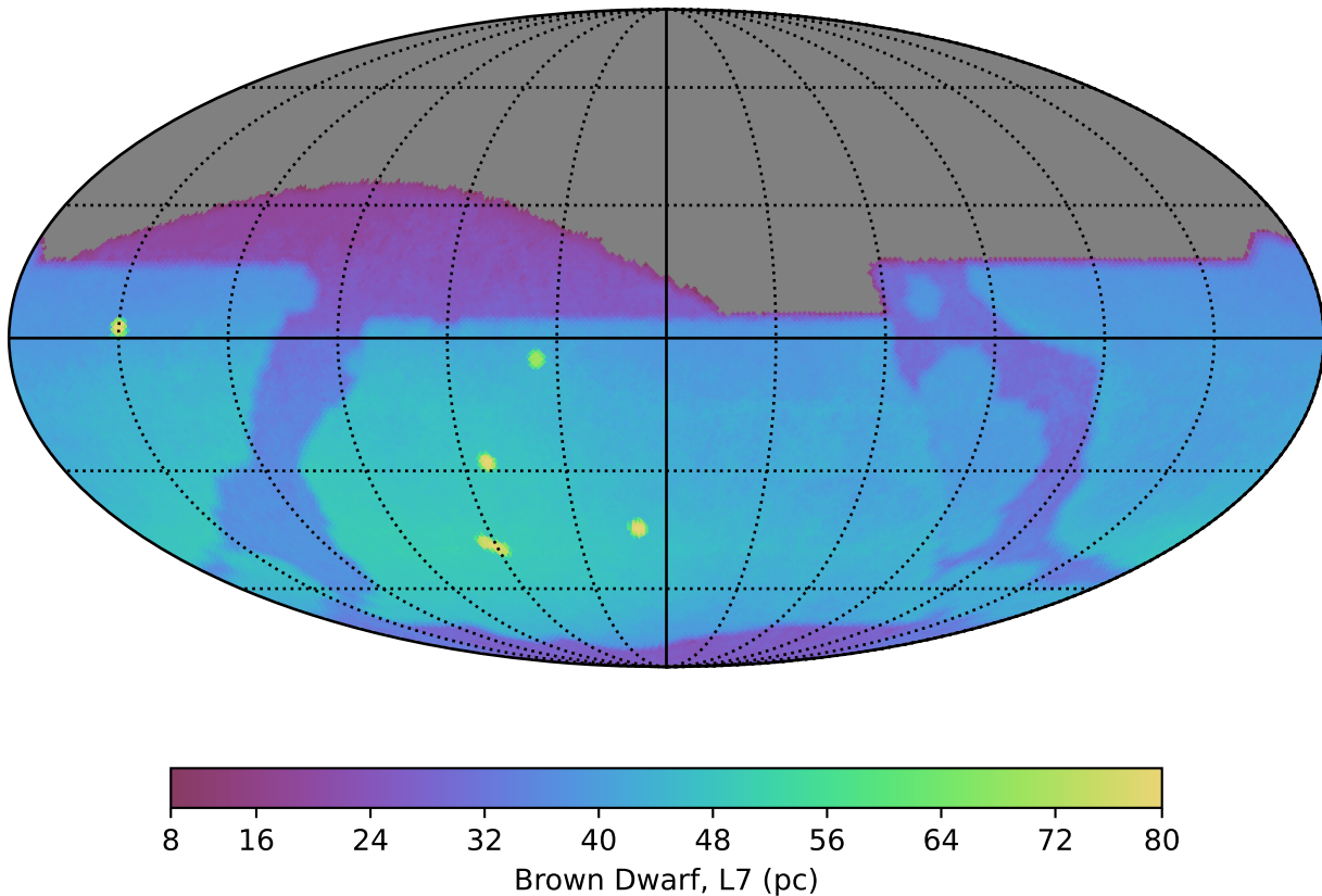
ddf_acor_sf10_lsf15_lsr20_v3.4_10yrs : Brown Dwarf, L7
