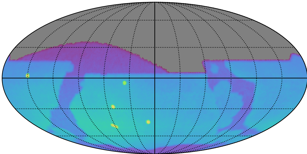
ddf_acor_sf10_lsf15_lsr20_v3.4_10yrs : Brown Dwarf, L4
