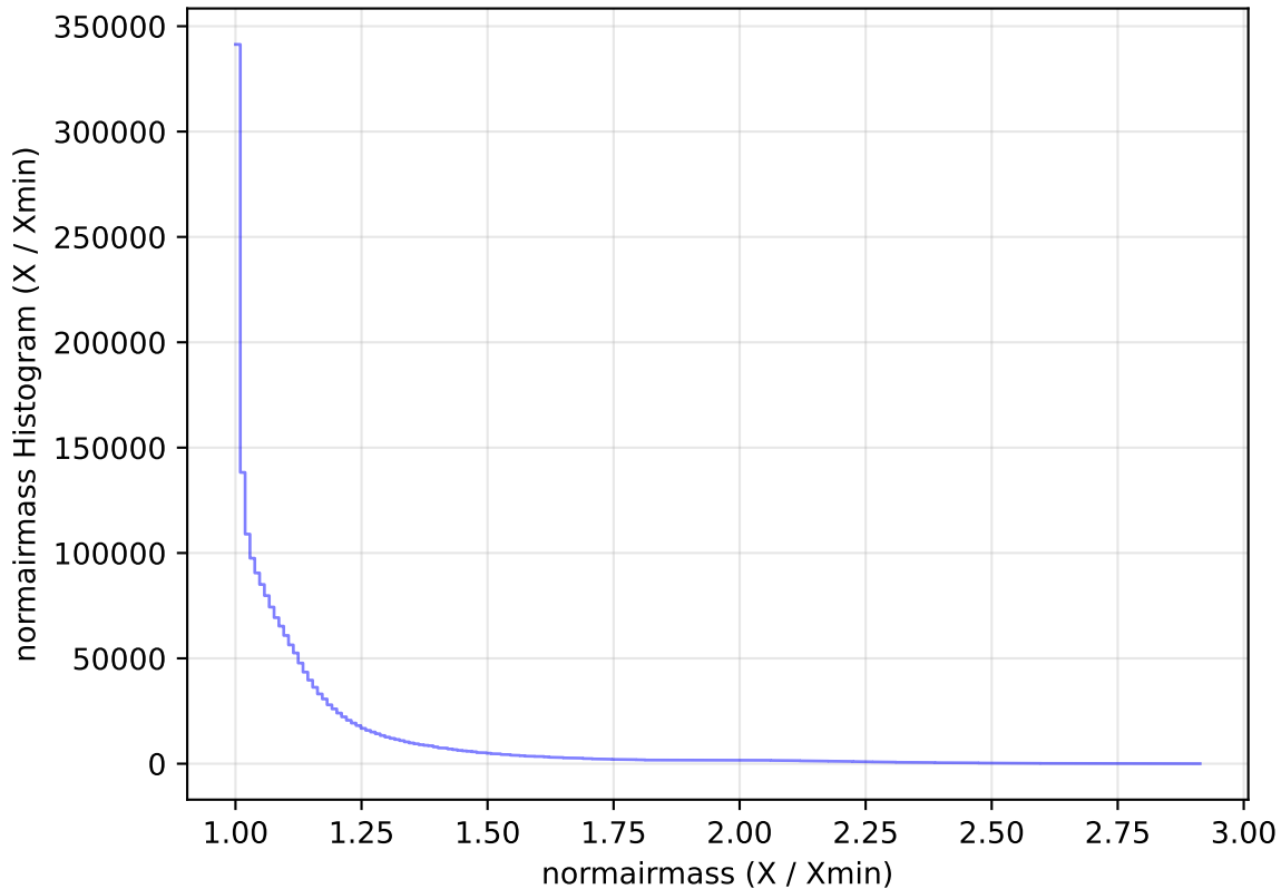
ddf_acor_sf10_lsf15_lsr20_v3.4_10yrs WFD all bands: normairmass Histogram
