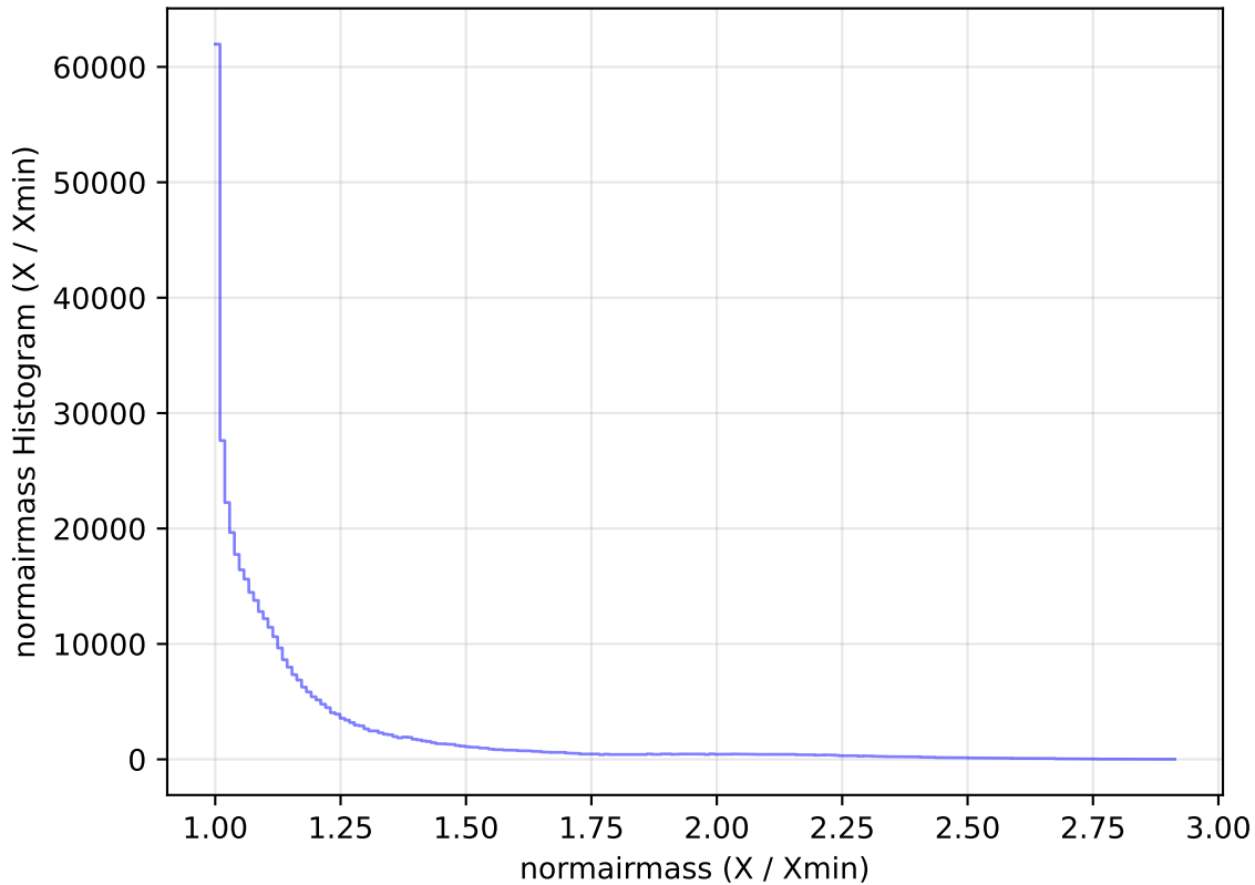
ddf_acor_sf10_lsf15_lsr20_v3.4_10yrs All sky z band: normairmass Histogram
