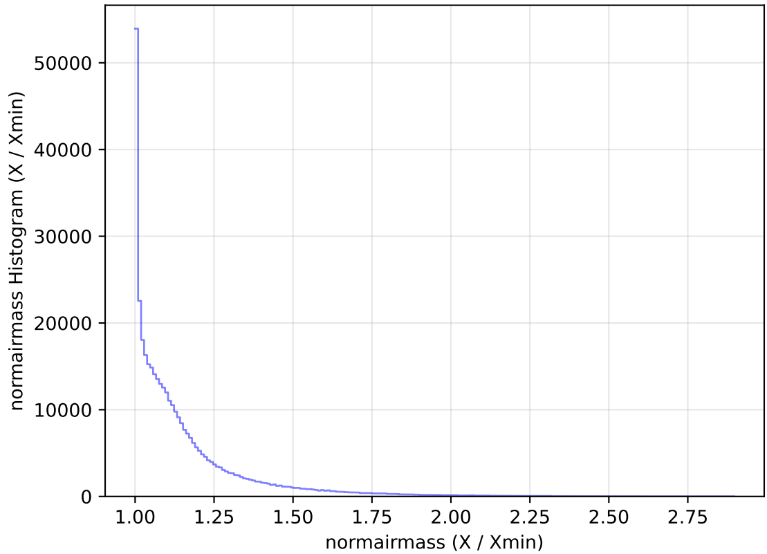
ddf_acor_sf10_lsf15_lsr20_v3.4_10yrs All sky y band: normairmass Histogram
