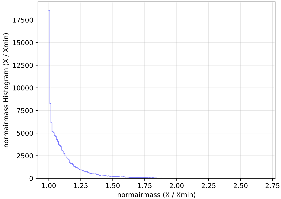
ddf_acor_sf10_lsf15_lsr20_v3.4_10yrs All sky u band: normairmass Histogram
