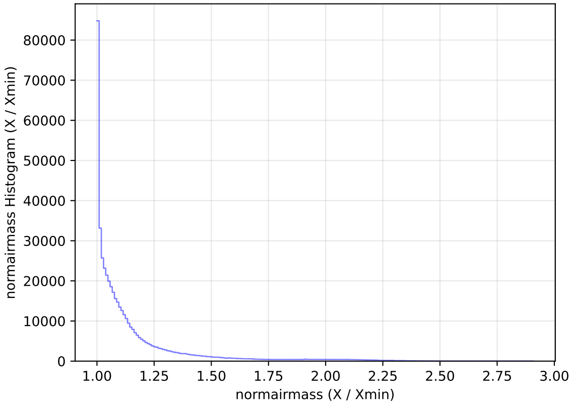
ddf_acor_sf10_lsf15_lsr20_v3.4_10yrs All sky r band: normairmass Histogram
