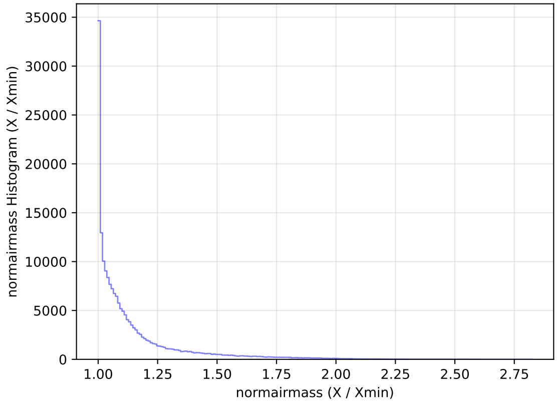
ddf_acor_sf10_lsf15_lsr20_v3.4_10yrs All sky g band: normairmass Histogram
