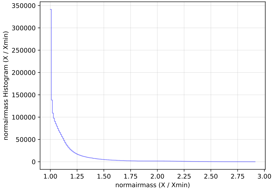
ddf_acor_sf10_lsf15_lsr20_v3.4_10yrs All sky all bands: normairmass Histogram
