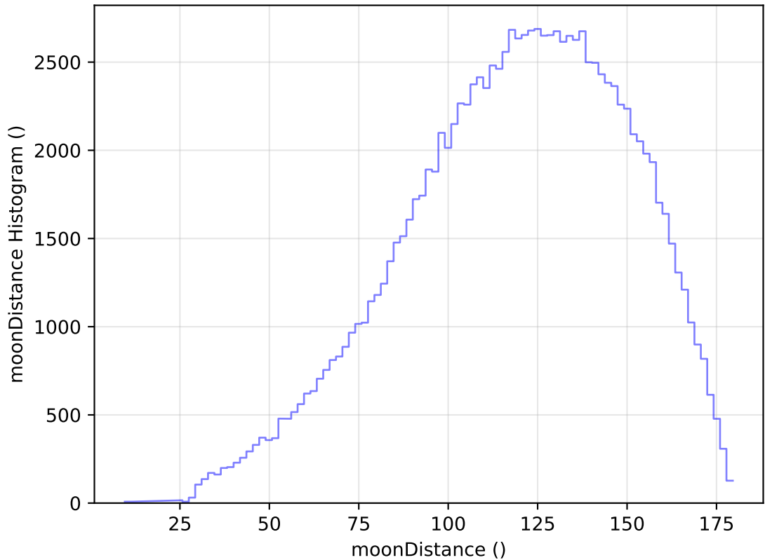
ddf_acor_sf10_lsf15_lsr20_v3.4_10yrs WFD u band: moonDistance Histogram
