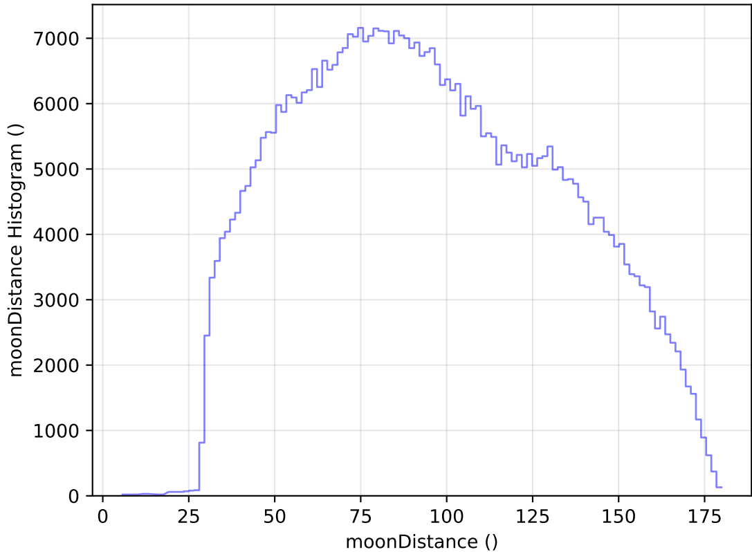
ddf_acor_sf10_lsf15_lsr20_v3.4_10yrs WFD i band: moonDistance Histogram
