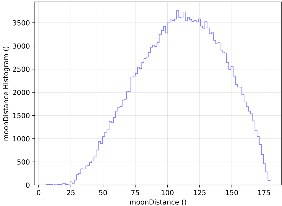
ddf_acor_sf10_lsf15_lsr20_v3.4_10yrs WFD g band: moonDistance Histogram
