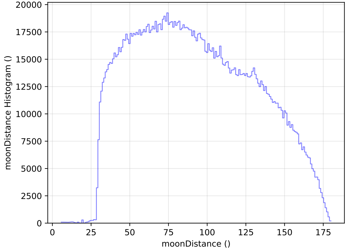
ddf_acor_sf10_lsf15_lsr20_v3.4_10yrs WFD all bands: moonDistance Histogram
