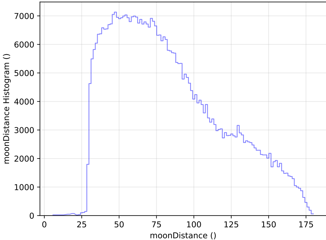
ddf_acor_sf10_lsf15_lsr20_v3.4_10yrs All sky z band: moonDistance Histogram
