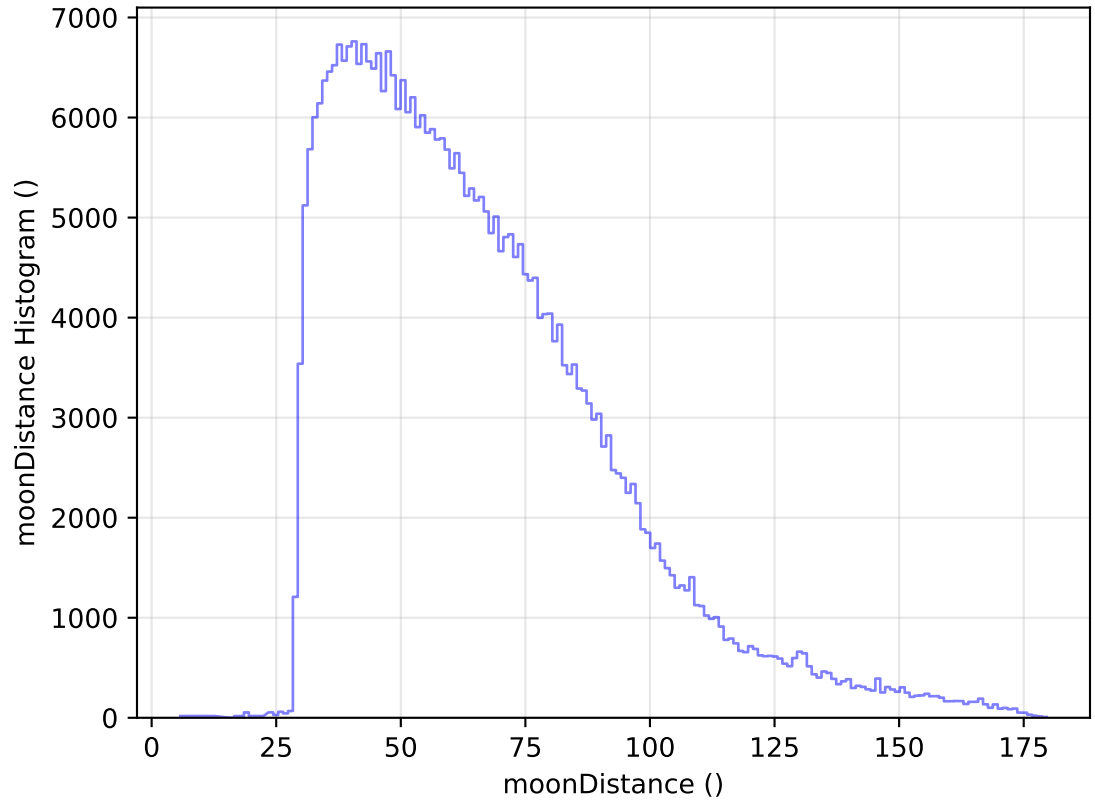
ddf_acor_sf10_lsf15_lsr20_v3.4_10yrs All sky y band: moonDistance Histogram
