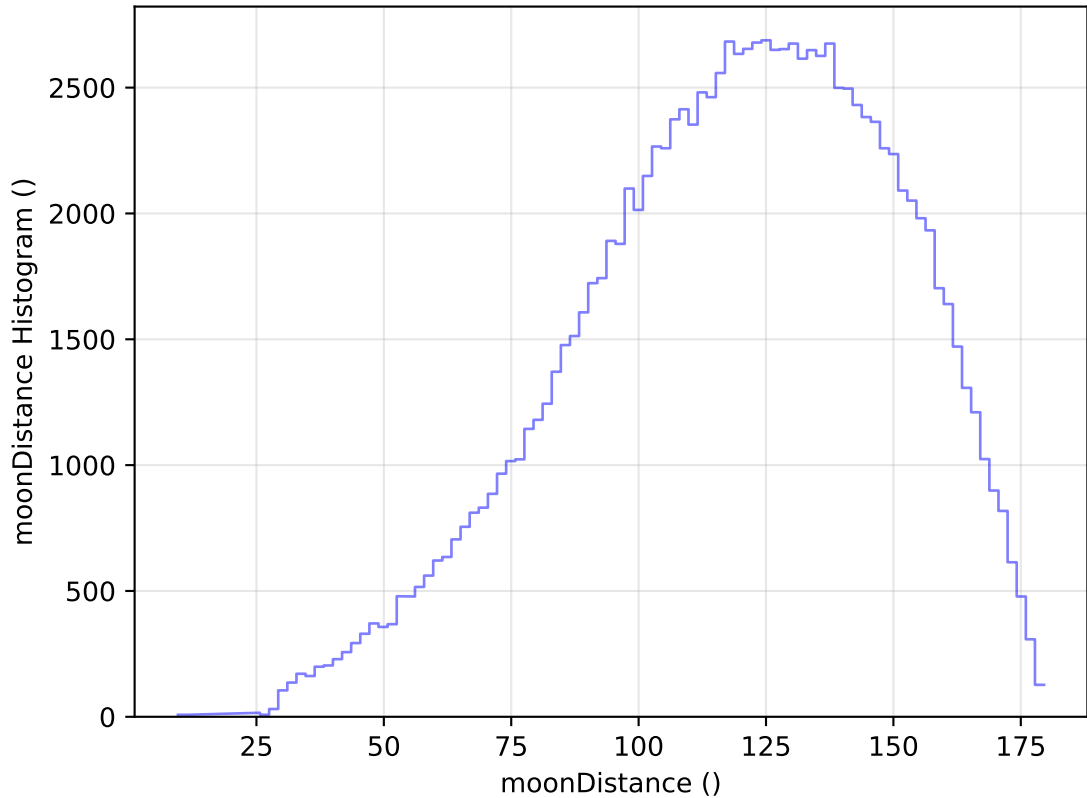
ddf_acor_sf10_lsf15_lsr20_v3.4_10yrs All sky u band: moonDistance Histogram
