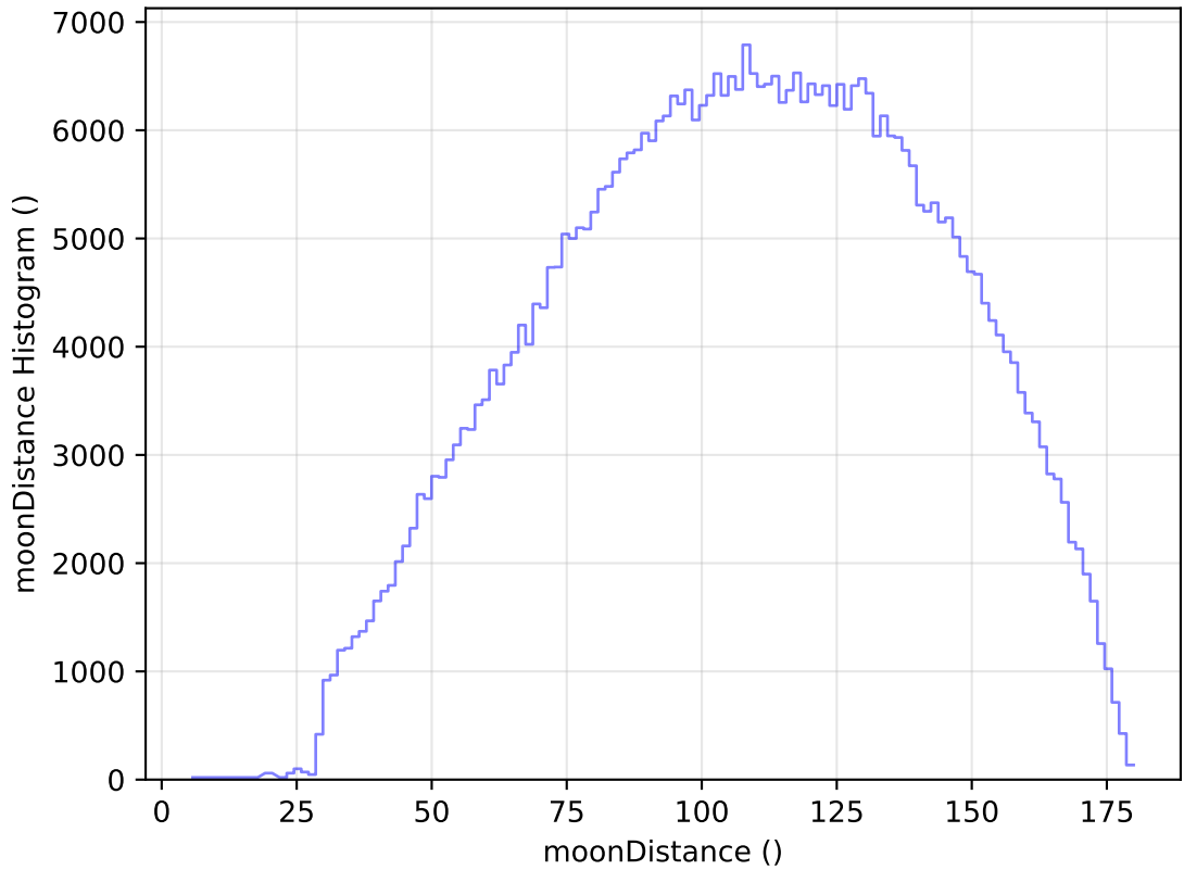
ddf_acor_sf10_ls15_lsr20_v3.4_10yrs All sky r band: moonDistance Histogram
