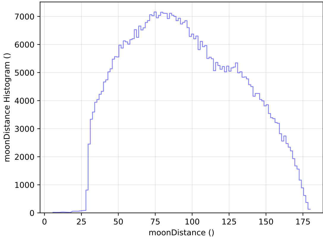
ddf_acor_sf10_lsf15_lsr20_v3.4_10yrs All sky i band: moonDistance Histogram
