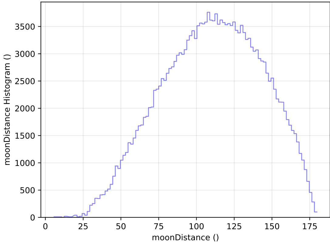
ddf_acor_sf10_lsf15_lsr20_v3.4_10yrs All sky g band: moonDistance Histogram
