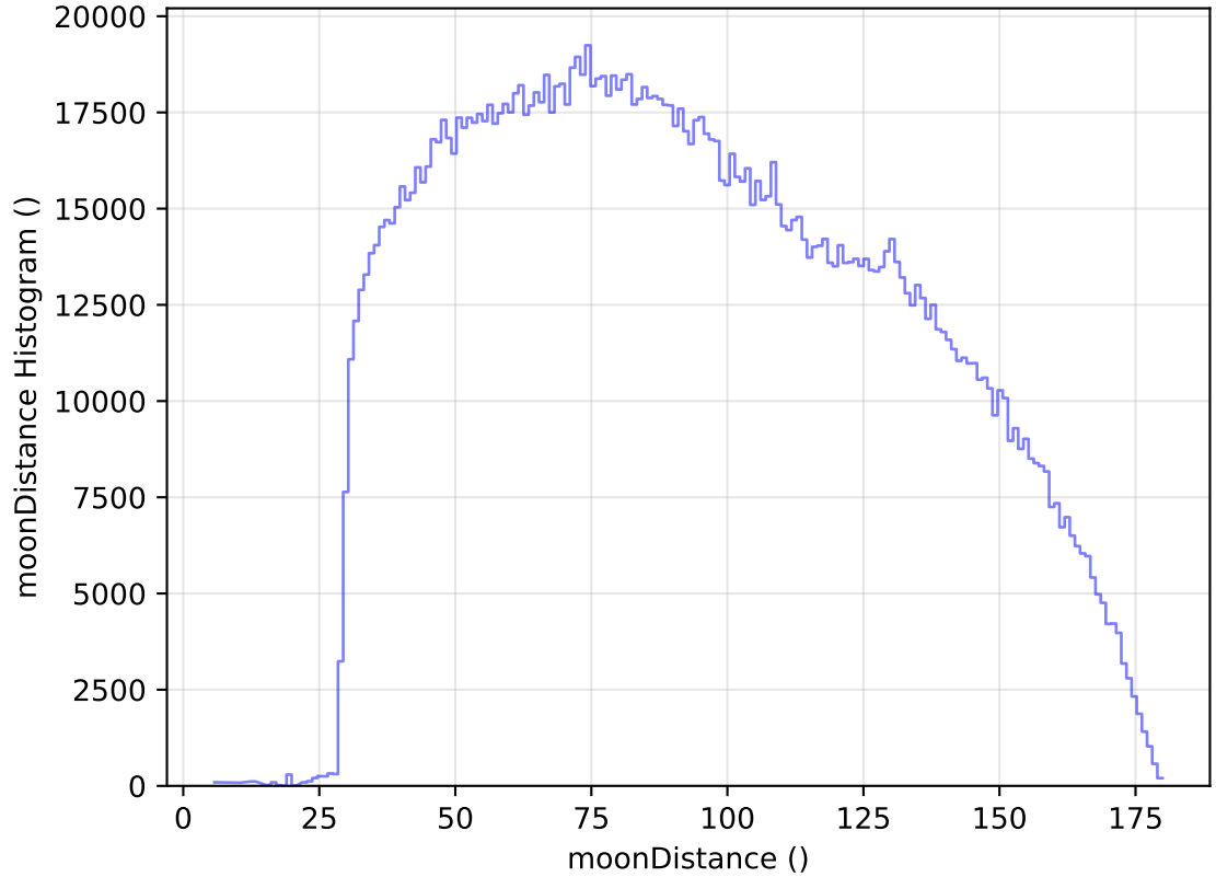
ddf_acor_sf10_lsf15_lsr20_v3.4_10yrs All sky all bands: moonDistance Histogram
