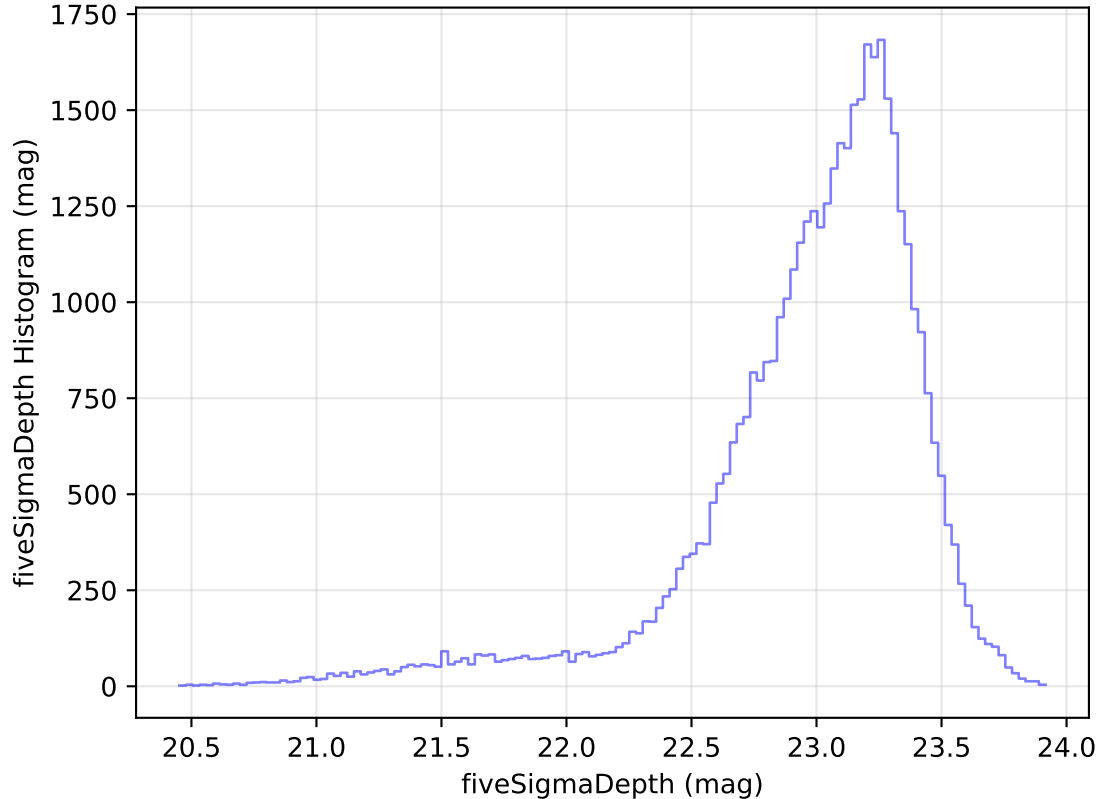
ddf_acor_sf10_lsf15_lsr20_v3.4_10yrs Yr 1 z band: fiveSigmaDepth Histogram
