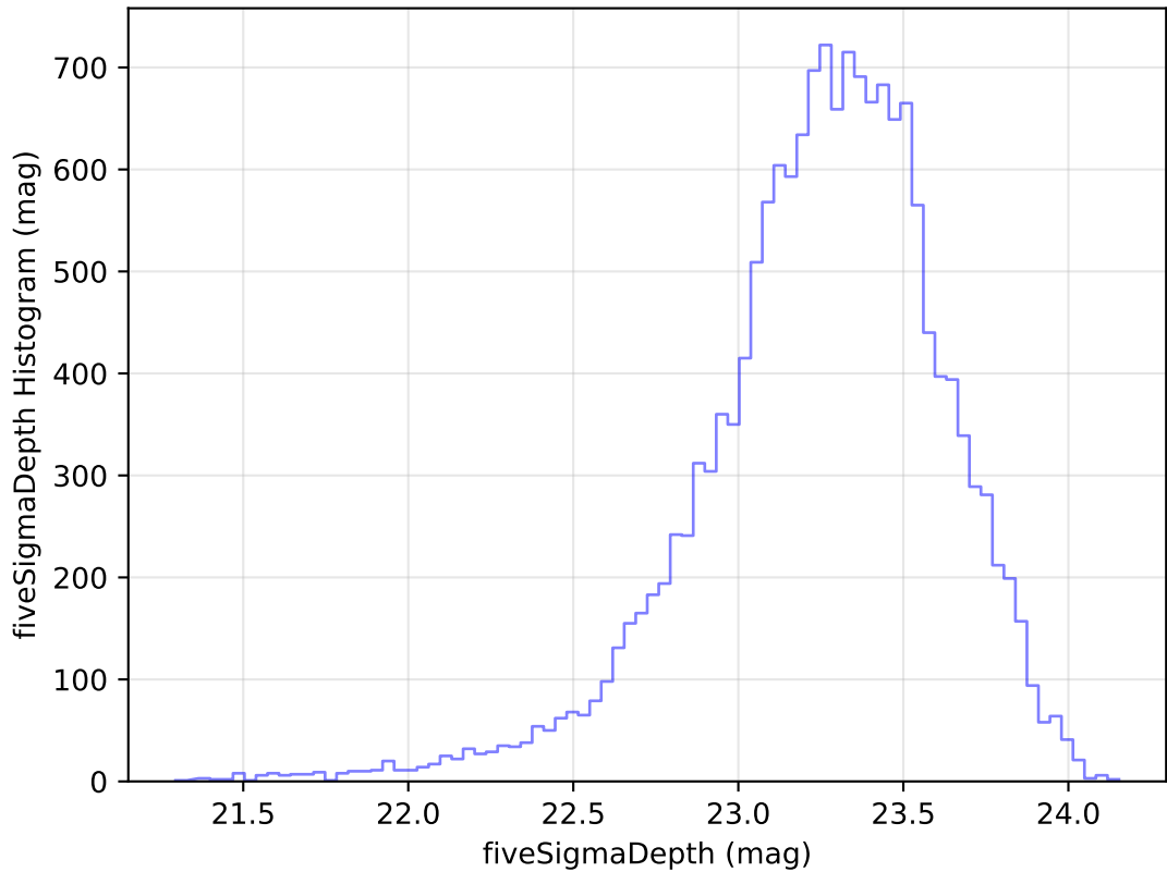
ddf_acor_sf10_lsf15_lsr20_v3.4_10yrs Yr 1 u band: fiveSigmaDepth Histogram
