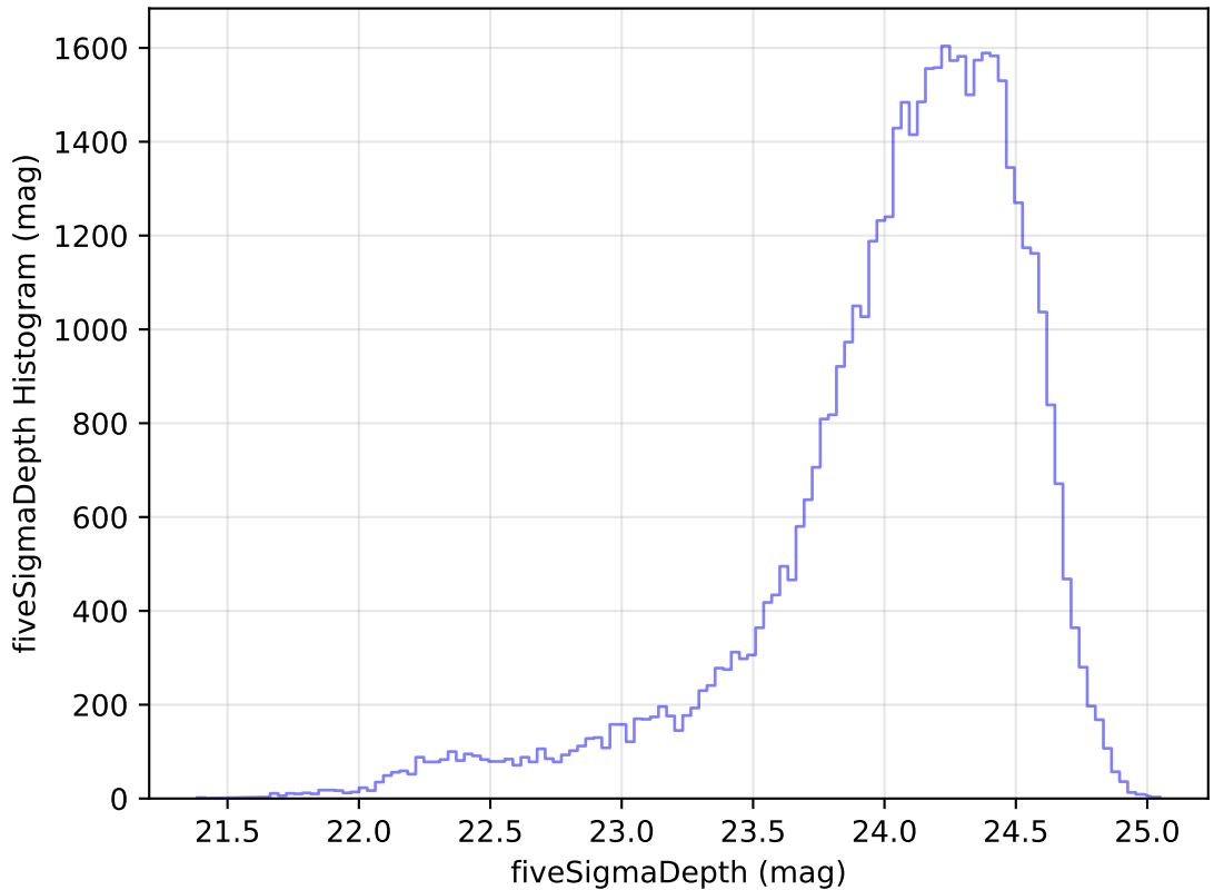
ddf_acor_sf10_lsf15_lsr20_v3.4_10yrs Yr 1 r band: fiveSigmaDepth Histogram
