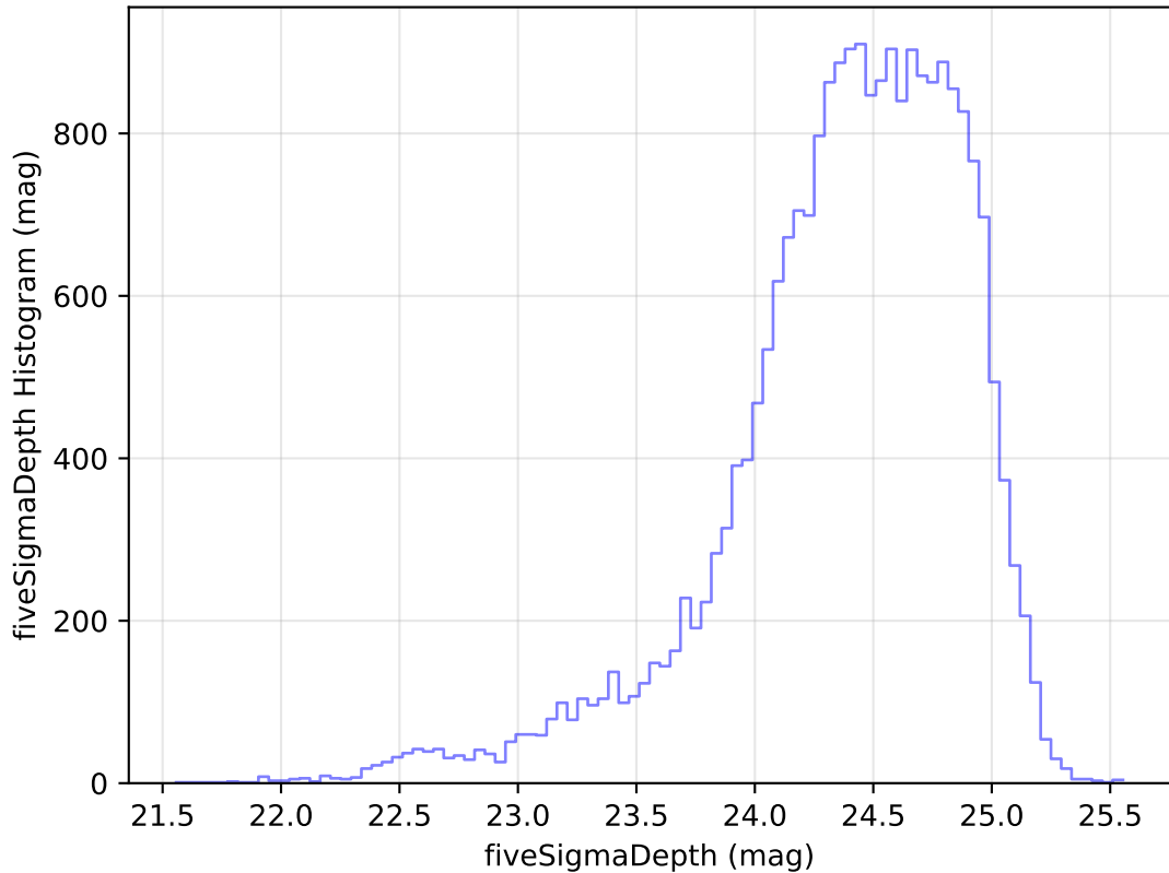
ddf_acor_sf10_lsf15_lsr20_v3.4_10yrs Yr 1 g band: fiveSigmaDepth Histogram
